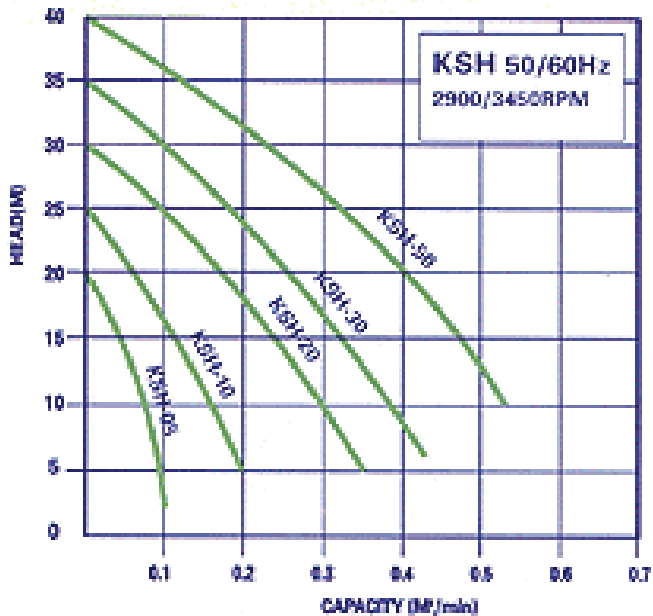
Performance Curve
